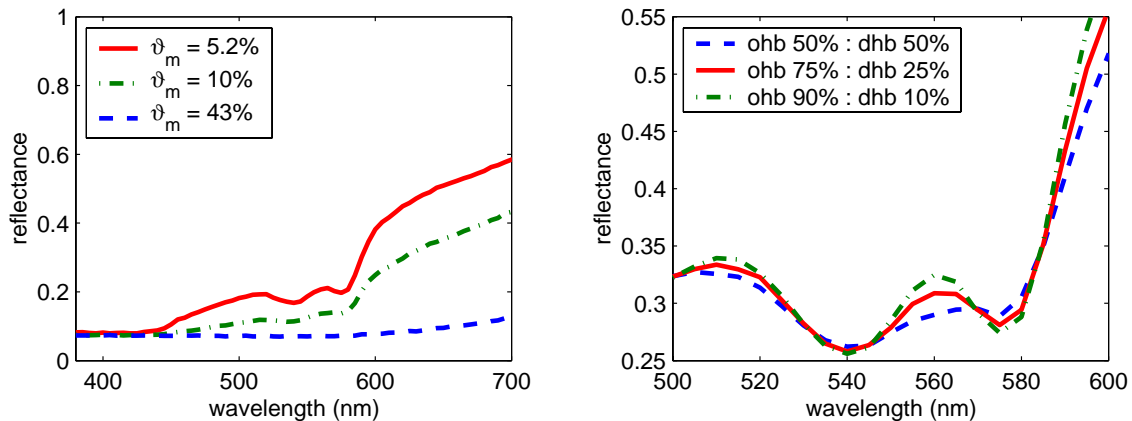
Figure 5: Comparison of modeled spectral curves provided by the BioSpec model ( \theta_i = 45^\circ ) considering the variation of biological parameters. Left: volume fractions of epidermis occupied by melanosomes ( \vartheta_m ). Right: ratio of oxygenated (ohb) to deoxygenated (dhb) hemoglobin in the dermal layers.
