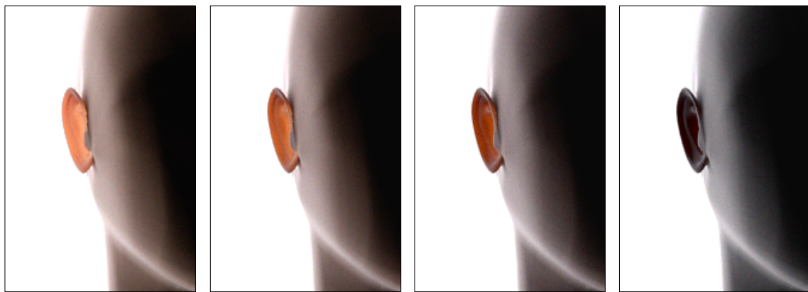
Figure 10: Images generated using the BioSpec model to show variations in the translucency of skin tissues associated with different levels of melanin pigmentation. From left to right: \vartheta_m = 1.9\% , \vartheta_m = 5.2\% , \vartheta_m = 12\% and \vartheta_m = 42\% .
