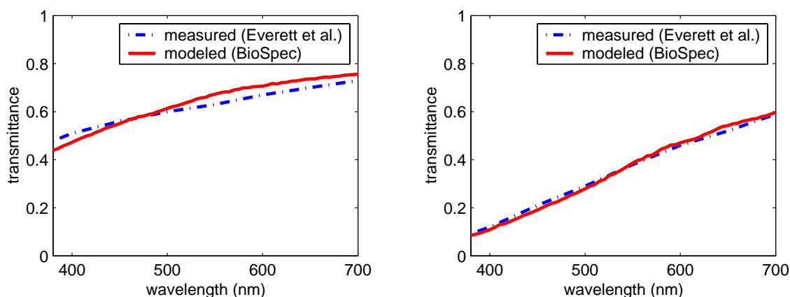
Figure 4: Comparison of modeled transmittance curves (for the stratum corneum and epidermis tissues) provided by the BioSpec model with actual measured curves provided by Everett et al. [1966]. Left: moderately pigmented specimen. Right: heavily specimen.
