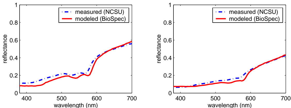
Figure 3: Comparison of modeled reflectance curves provided by the BioSpec model with actual measured curves available in the NCSU spectra database by Vrhel [1994]. Left: lightly pigmented skin specimen (NCSU file 113). Right: moderately pigmented specimen (NCSU file 82).
