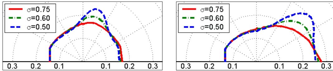
Figure 7: Comparison of modeled spectral curves provided by the BioSpec model considering variations on the aspect ratio ( \sigma ) of the stratum corneum folds. Left: \theta_i = 15^\circ . Right: \theta_i = 45^\circ .
