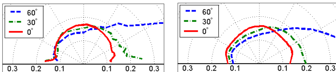
Figure 6: Comparison of BRDF curves for a lightly pigmented specimen. Left: actual measured BRDF curves provided by Marschner et al. [1999]. Right: modeled BRDF curves provided by the BioSpec model.
